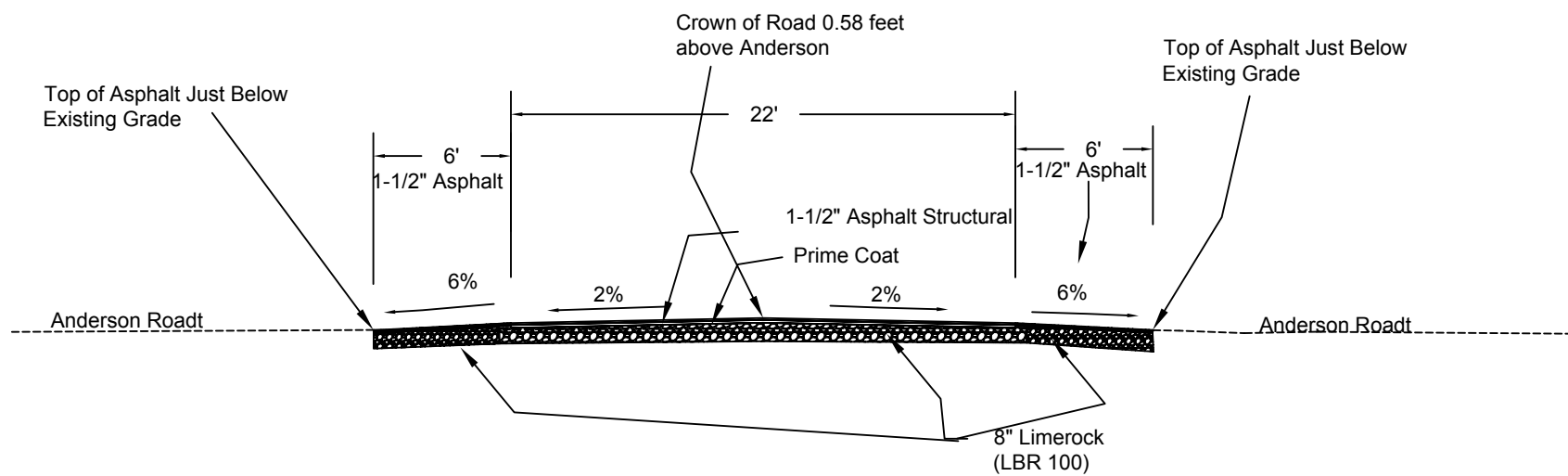
TYPICAL ROADWAY SECTION Anderson Road
