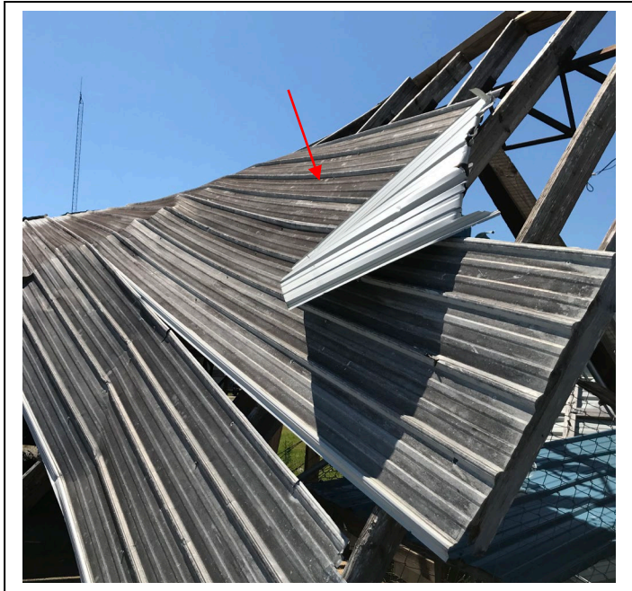
Approximately, 2960 SF of AG roof panel was uplifted and torn off by high winds
