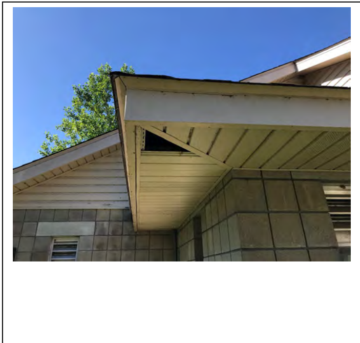
Second soffit vinyl piece missing. 1FT (L) X 1FT (W).
