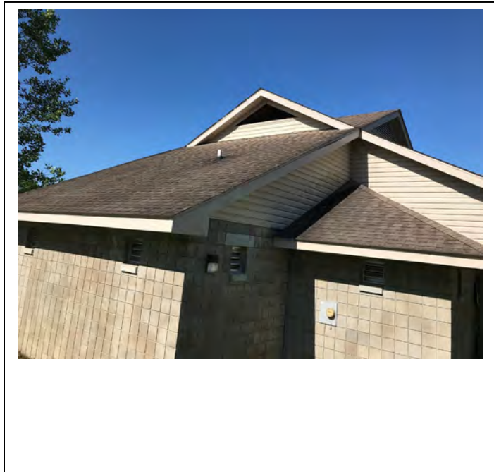
Gable vent blown out. 4FT (L) X 3FT (W).
